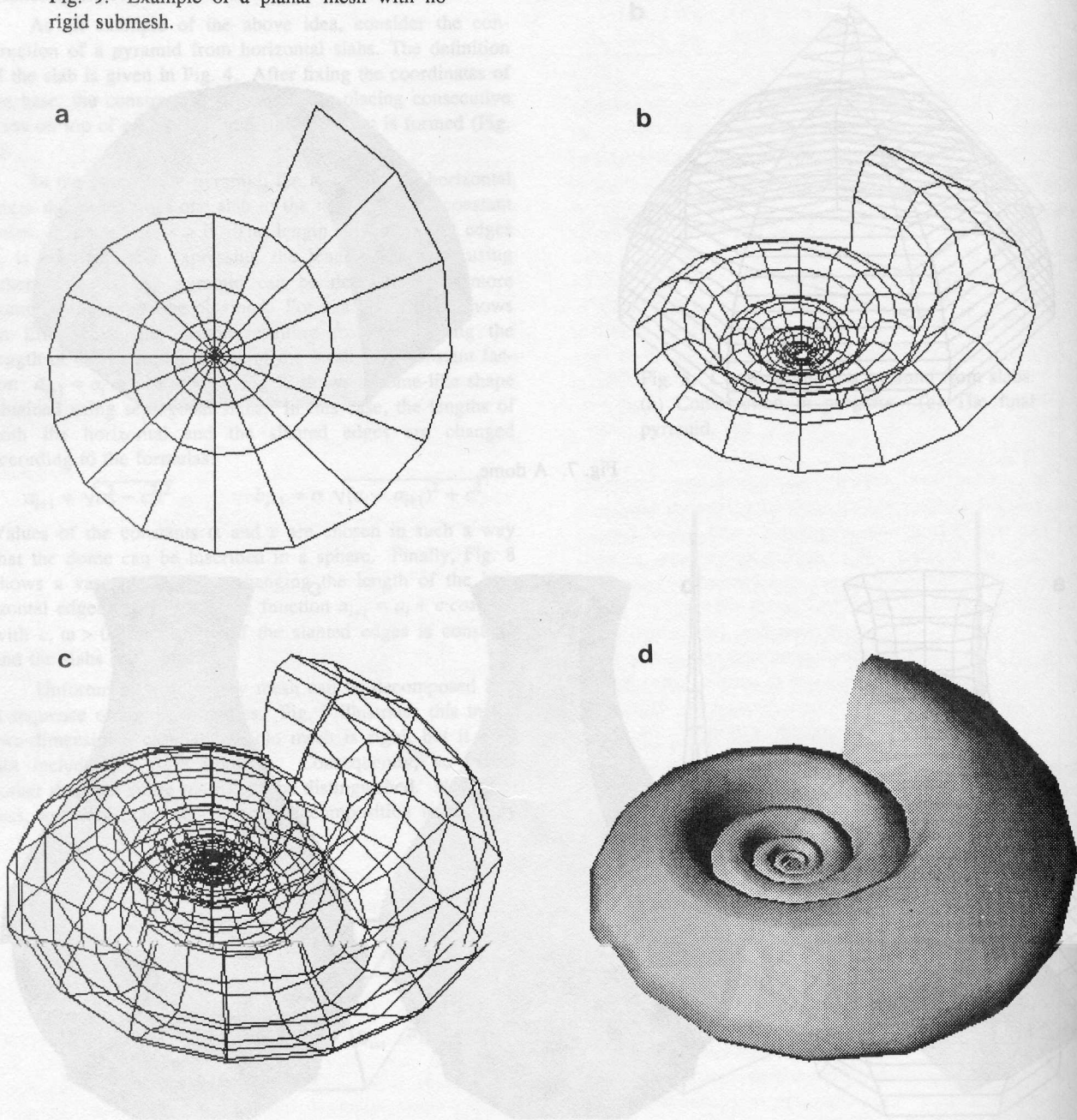
Fig. 10. Construction of a shell.
