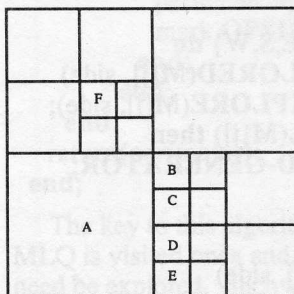
Fig. 1. An Adjacency Configuration.
