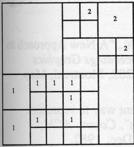
Fig. 5. Labels Resulting From Phase 5.
