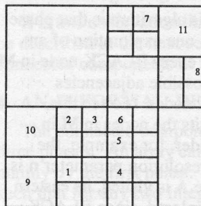
Fig. 3. Decomposition of Fig. 2.
