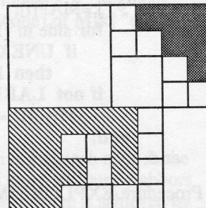
Fig. 2. A Region With 2 Components.
