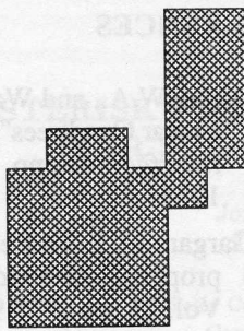
Fig. 6. A Connected Region.
