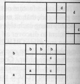
Fig. 4. Results of Phase 1.
