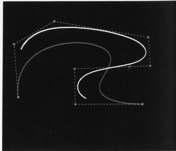
Colour Plate 2: Two splines that share a common control polygon (shown in green), but have different evaluation routine attributes. The white curve is a uniform cubic B-spline, and the red curve is a seventh degree Bézier curve.
