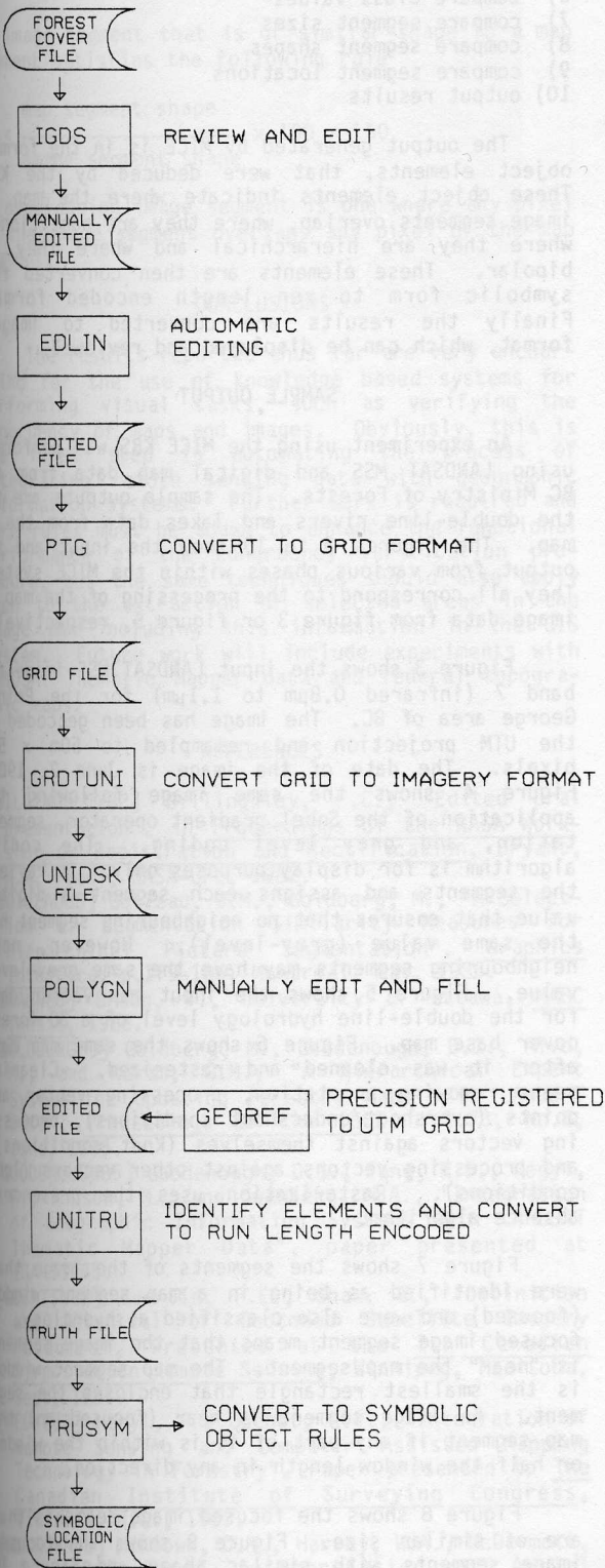
FIGURE 1: THE PROCEDURE FOR PREPROCESSING THE CARTOGRAPHIC INFORMATION
