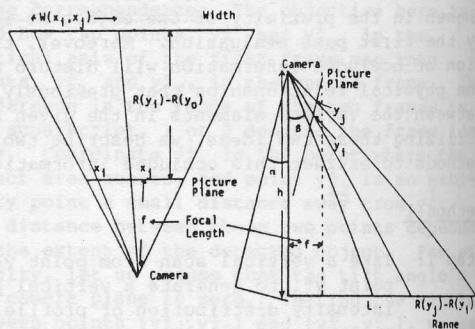
(a) Mapping of Width (b) Mapping of Range
