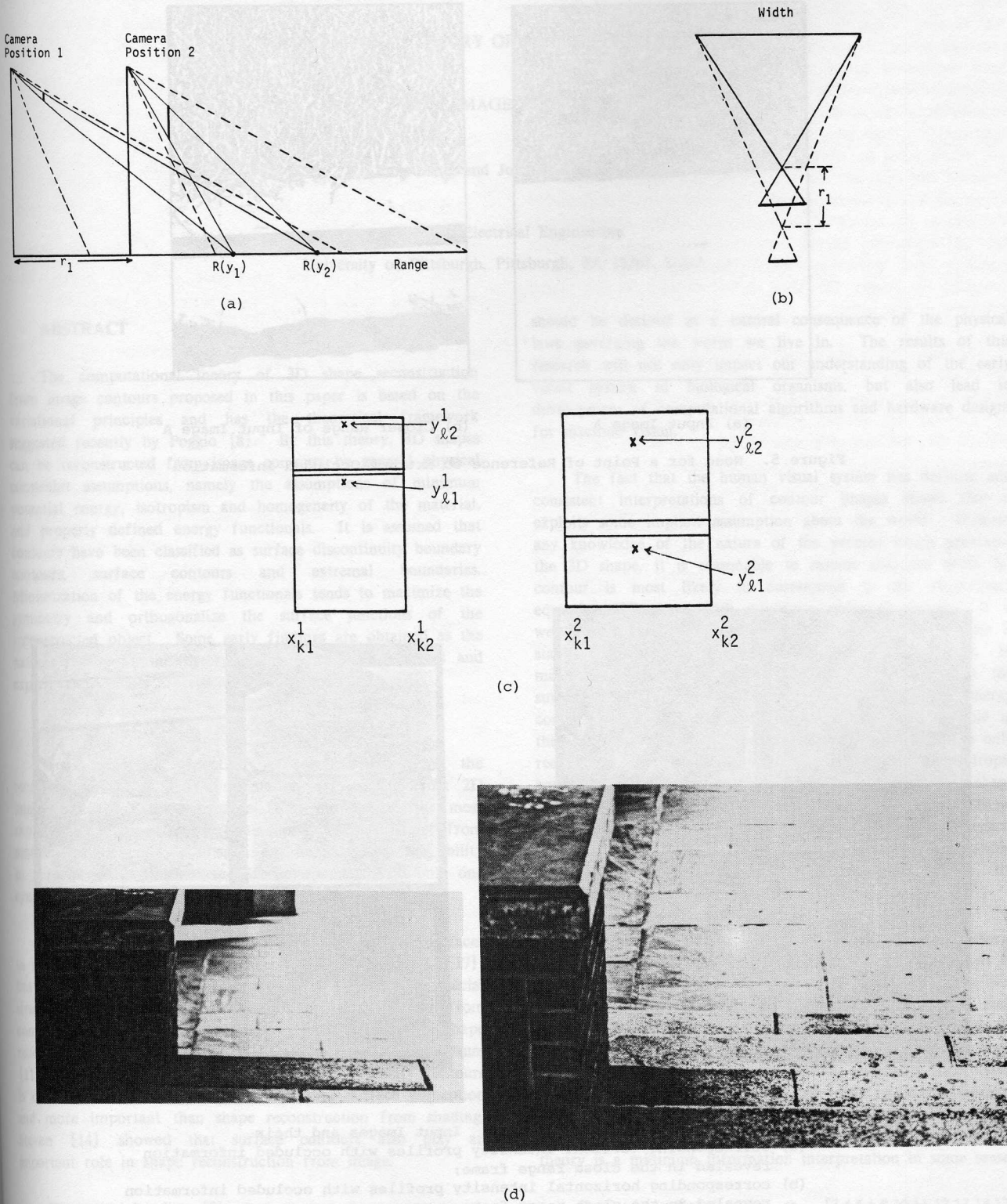
Figure 4. Image Correspondence for Extracting Occluded Information. (a) Correspondence in Range; (b) Correspondence in Width; (c) Mapping the Reference Points; (d) Mapping the Location of Interest.
