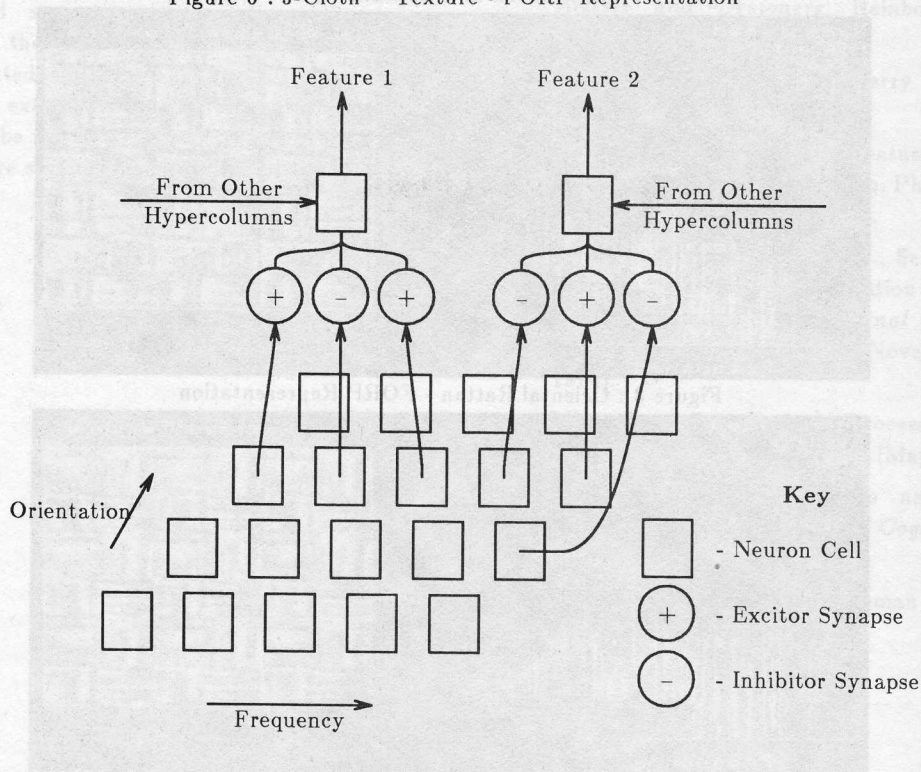
Figure 7 : Simplified Model of Hypercolumn Feature Extraction
