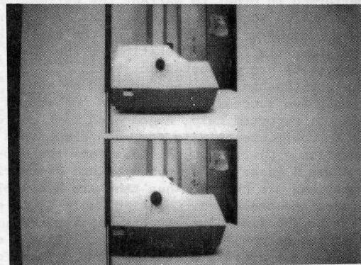
Fig.4: "Printer" sequence
