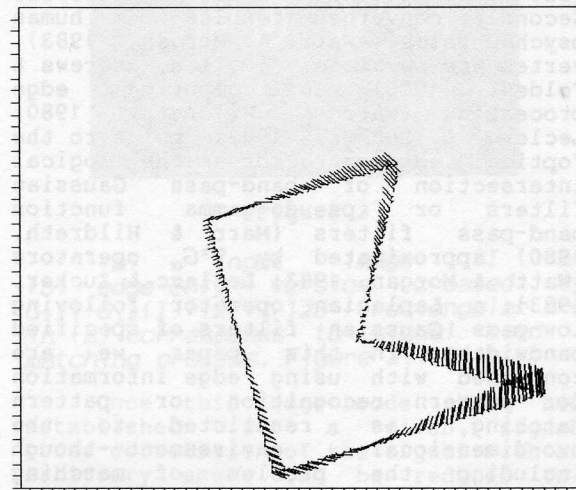
Fig.7c: Resulting complete displacement field
