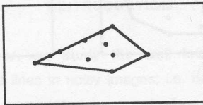
Figure 2: A Typical Hull h_k .
