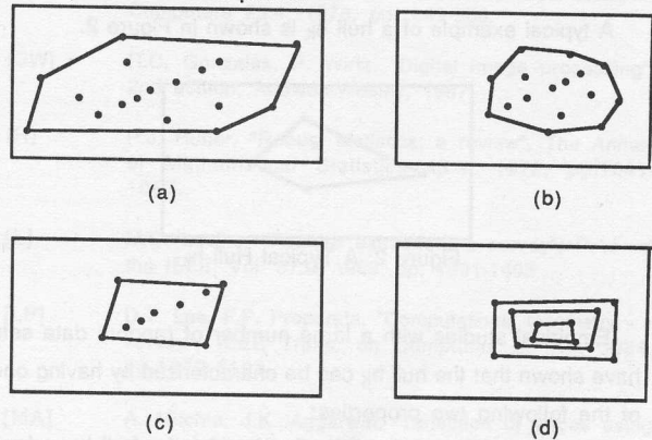
Figure 1: Using Convex Hulls for Noise Removal (a) Initial Case for Line Segment (b) Subsequent Case for Line Segment and Initial Case for Lines (c) A Case Where as Many Points as Noise Points are Removed (d) A Worst Case Scenario
