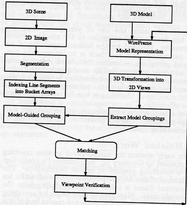
Figure 1: The framework of our motion tracking system. Model-Guided Groupings are incorporated as our matching tokens.
