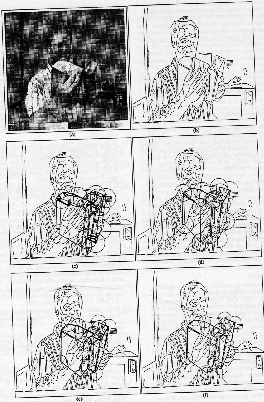
Figure 6: Matching refinement with model-guided junction groupings. The original image from a motion sequence (a). Line segments are formed in (b). Superimposed model edges are projected from its prior estimated viewpoint. Nearby are top ranked matching edges. Heavy bars are the perpendicular errors to be minimized. Junction groupings are formed within each circle. Searching regions (circles) will be reduced in consecutive iterations (c)-(f).
