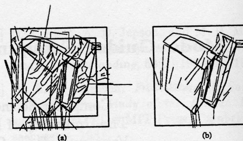
Figure 2: (a) Local Focus Window is an extended bound around the superimposed model edges. (b) Compatible image edges are selected after passing all the unary constraints.
