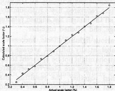
Figure 4: Plot of the actual scale factors versus the calculated ones.
