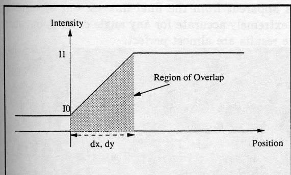
Figure 2: Blending function used to eliminate intensity differences between images.
