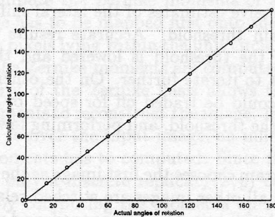
Figure 3: Plot of the actual angles of rotation versus the calculated ones. All angles are in degrees.
