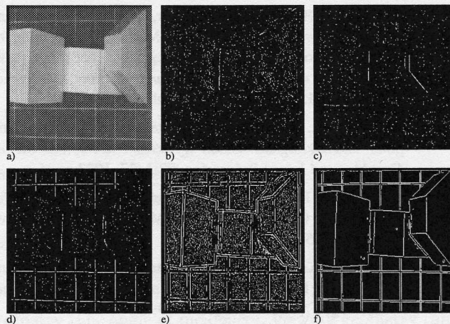
Figure 13: a) Polyhedric image. b) Staircase. c) Valley. d) Roof. e) Concave slope and convex slope. f) Step. The scale used is \sigma = 1 .
