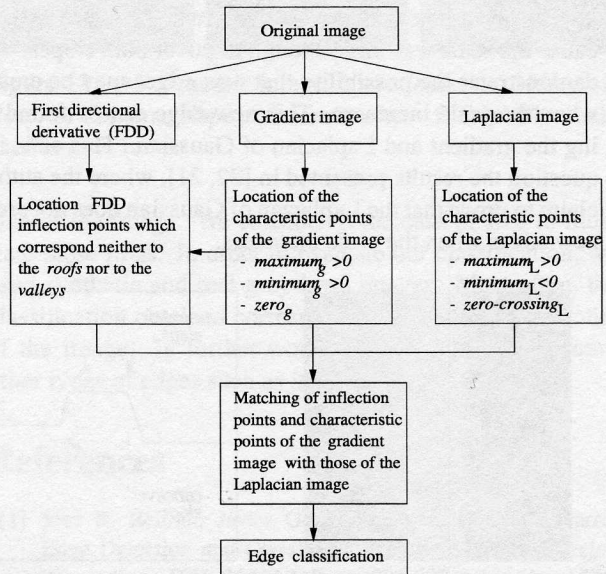
Figure 8: General algorithm for detection and classification of edges.
