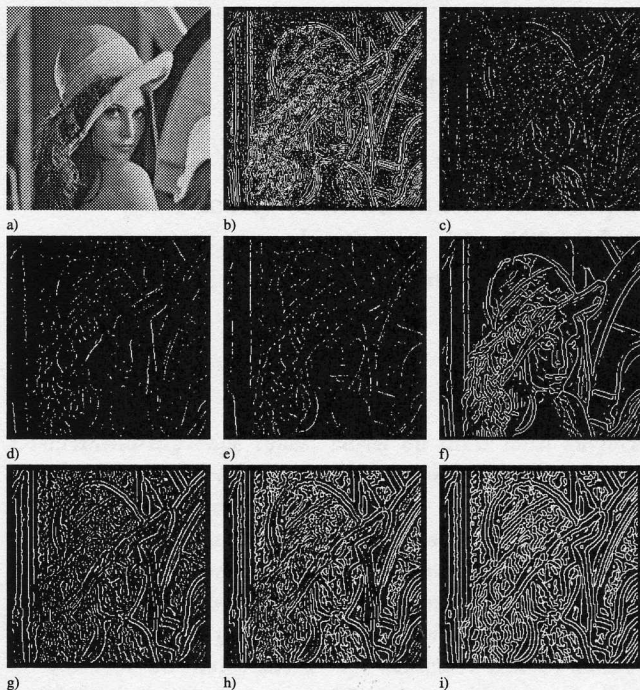
Figure 12: a) Image of Lenna. b) All types of edges, at \sigma = 1.5 . c) Staircase. d) Roof. e) Valley. f) Step. g) Concave slope and convex slope. h) Slopes which are neither roofs nor valleys. i) All slopes without classification.
