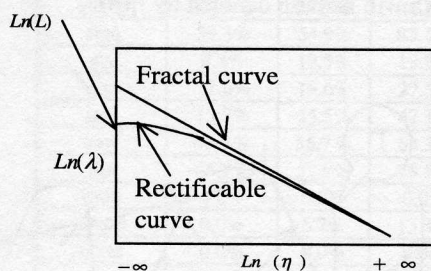
Figure 1.2 : fractal curve
