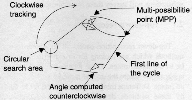
Figure 1: Tracking the outline of an object.
