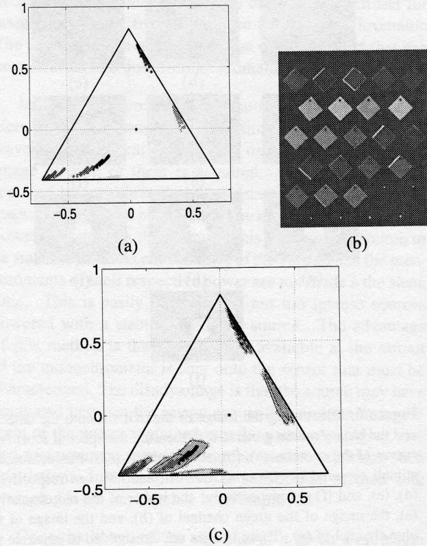
Figure 9: (a) Traces of predicted colors under daylight for the various samples on the chart shown in (b). (c) Detection regions used for pixel classification.
