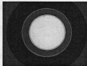
Figure 2: Image of the reflectance standard (white disk at the center) having an 80% reflectance as seen by the red channel of the camera. The darker annulus around the standard is the light source seen from the back, see Fig. 1.
