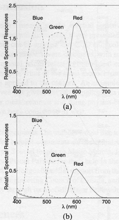
Figure 7: Spectral sensitivity curves for the camera characterized with an objective. These were obtained by scanning the spectrum at 10 nm intervals between 400 nm and 700 nm. In (a) color balancing has been performed, whereas this is not the case in (b) where the curves are those of the factory settings.
