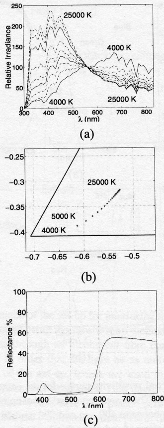
Figure 8: (a) Spectral distributions of daylight with correlated color temperatures ranging from 4000 °K to 25000 °K in steps of 1000 °K obtained from the model of Judd et al. [9]. (b) Trace of predicted color points using Eq. 11 for a material with red appearance having the spectral reflectance shown in (c).
