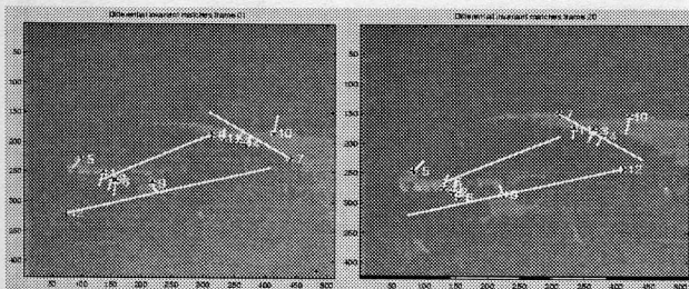
Figure 1: Greylevel differential invariant matches. Left image is frame 01 and right image is frame 20. Matches 7, 8 and 12 are incorrect.
