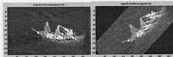
Figure 9. Lockheed sequence epipolar lines for frames 00 and 08.
