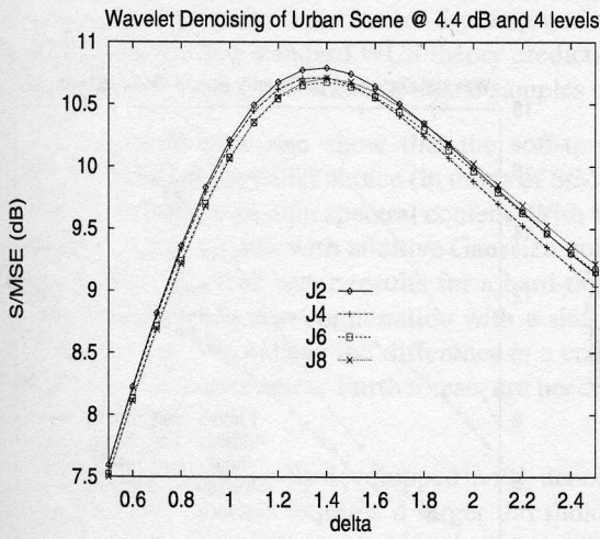
Figure 4: Wavelet denoising of the urban scene @ 4.4 dB and 4 levels
