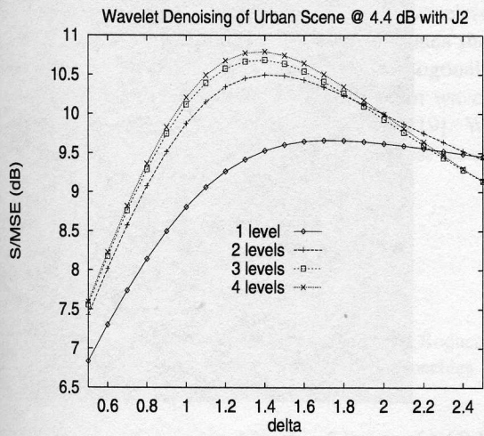
Figure 5: Wavelet denoising of the urban scene @ 4.4 dB with J2
