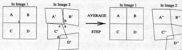
Figure 3: A,B,C and D are four patches of image 1 and A' , B' , C' and D' are their corresponding patches in image 2. The average step forces some patch vertices to coincide if they are enough close from each others. A'' , B'' , C'' , and D'' are the result of the averaging step. Note that this step improves but can not solve all cases of intersecting patches (e.g. C'' with D'' ).
