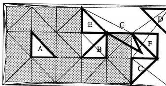
Figure 7: Gray triangles are matched triangles and the topology of their set is the same in the two images. Black framed triangles A,B,C and D (resp. E,F,G) are (resp. are not) correct input for the InsertMatchedTriangle operator. Thus, triangle A,B,C can be added in both images to the current structure as matched triangles. Triangles E and F violate the topological restriction. One edge of Triangle G intersects an edge of the contour.
