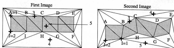
Figure 6: A,B...J are the matched vertices of gray and matched triangles in the two images. A new point match is consistent if its two points are corresponding vertices of a match of the contour, or are both outside of the set of matched triangles. Matches 2 and 4 are consistent but 1,3 and 5 are not. Note that match 4 is consistent even though the matching ordering constraint is violated (see the ball in Figure 1).
