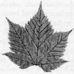
Figure 6: Veins of a Leaf
