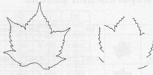
Figure 11: Teeth of A Leaf
