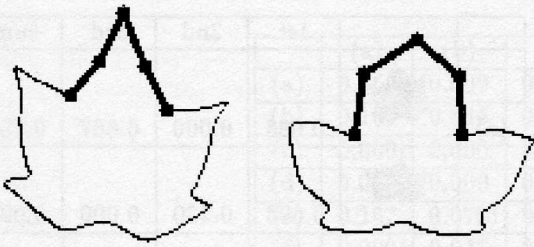
Figure 10: Polygonal Approximation of A Mid-Most Piece of A Leaf
