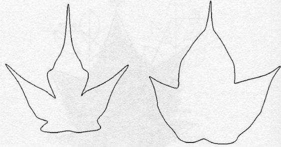
Figure 8: Normalized Shapes of Leaves
