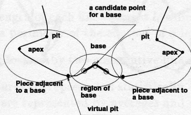
Figure 4: A Bottom of a Leaf
