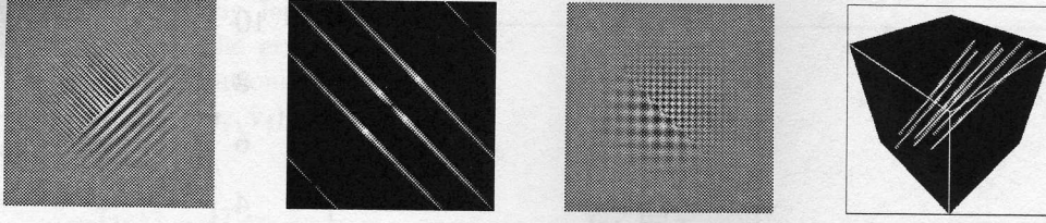
Figure 2.1: (from left to right): a) Gaussian-windowed 1D signal with sinusoids acting as occluding and occluded surfaces. The occluding signal has spatial frequency k_1 = \frac{2\pi}{16} and velocity \mathbf{v}_1 = (1, 1) . The occluded signal has frequency k_2 = \frac{2\pi}{8} and velocity \mathbf{v}_2 = (-1, 1) . b) Fourier spectrum of a) . c) Gaussian-windowed 2D signal with sinusoids acting as occluding and occluded surfaces. The occluding signal has spatial frequency \mathbf{k}_1 = (\frac{2\pi}{16}, \frac{2\pi}{16}) and velocity \mathbf{v}_1 = (1, 1, 1) . The occluded signal has frequency \mathbf{k}_2 = (\frac{2\pi}{8}, \frac{2\pi}{8}) and velocity \mathbf{v}_2 = (-1, -1, 1) . d) Fourier spectrum of c) .
