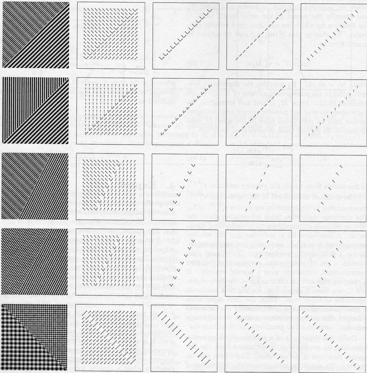
Figure 4.4: Synthetic imagery and results with \mathbf{k}_1 and \mathbf{v}_1 occluding. (top to bottom): 1D imagery a) k_1 = \frac{2\pi}{16} , k_2 = \frac{2\pi}{8} , \mathbf{v}_1 = (1, 1) and \mathbf{v}_2 = (-1, 1) . b) k_1 = \frac{2\pi}{16} , k_2 = \frac{2\pi}{8} , \mathbf{v}_1 = (1, 1) and \mathbf{v}_2 = (0, 1) . c) k_1 = k_2 = \frac{2\pi}{16} , \mathbf{v}_1 = (0.5, 1) and \mathbf{v}_2 = (-1, 1) . d) k_1 = k_2 = \frac{2\pi}{16} , \mathbf{v}_1 = (0.5, 1) and \mathbf{v}_2 = (-0.75, 1) . e) 2D imagery \mathbf{k}_1 = (\frac{2\pi}{16}, \frac{2\pi}{16}) , \mathbf{k}_2 = (\frac{2\pi}{8}, \frac{2\pi}{8}) , \mathbf{v}_1 = (1, 1, 1) and \mathbf{v}_2 = (-1, -1, 1) . (left to right): a) Synthetic image. b) Optical flow. c) Multiple velocities. d) Occluding velocities. e) Occluded velocities.
