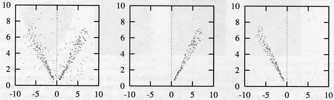
Figure 3.3: a (left): Mixture of two angular normals randomly generated with \pi_0 = 0.20 , \pi_1 = 0.40 , \pi_2 = 0.40 , \mathbf{v}_1 = (1, 1) , \mathbf{v}_2 = (-1, 1) and \sigma_v = 0.075 radians. b) (center): EM results for observations with \tau_{1j} > 0.95 and c) (left): with \tau_{2j} > 0.95 . The algorithm converged to \pi_0 = 0.182 , \pi_1 = 0.411 , \pi_2 = 0.406 , \mathbf{v}_1 = (1.017, 1) and \mathbf{v}_2 = (-1.022, 1) in 15 iterations. Measurements at a distance \lambda = 2.5 standard deviations are considered as outliers.
