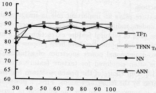
Figure 2. Recognition rates of TF , TFNN , NN , and ANN on test samples.
