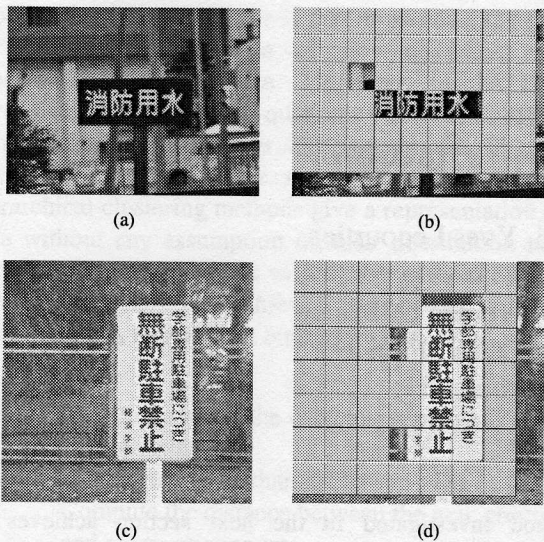
Figure 4. Recognition results of some test images. (a) and (c) test images; (b) and (d) results of applying TFNN to (a) and (c).
