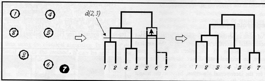
Figure 4 : The new element moves two sub-trees away
