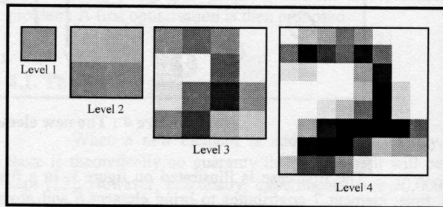
Figure 5 : Representation of a 2 using a 4 level resolution pyramid
