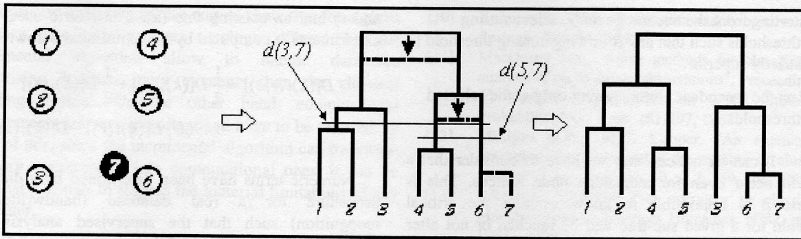
Figure 3 : The new element brings two sub-trees nearer
