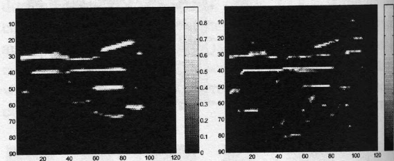
Figure 9: Correlation matrices, image WoBA. (left) intensity data; (right) invariant representation.
