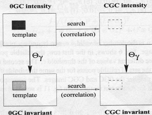
Figure 7: The template location problem: A query template is cut out from the 0GC intensity image and correlated with the corresponding CGC intensity image. We test if the correlation maximum occurs at exactly the same location as in the 0GC intensity image. The same process is repeated with the invariant representations of the 0GC and CGC images.
