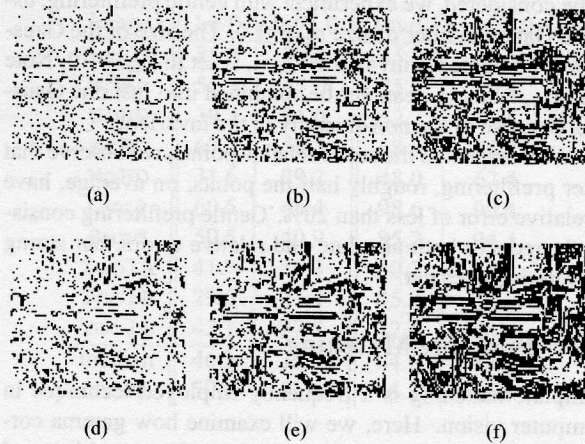
Figure 6: Reliable points RP_\epsilon for invariant \Theta_{m12\gamma} , in black, image w0BA, without and with pre-filtering. (a) \sigma_{pre}=0 , \epsilon=5.0 ; (b) \sigma_{pre}=0 , \epsilon=10.0 ; (c) \sigma_{pre}=0 , \epsilon=20.0 ; (d) \sigma_{pre}=1.0 , \epsilon=5.0 ; (e) \sigma_{pre}=1.0 , \epsilon=10.0 ; (f) \sigma_{pre}=1.0 , \epsilon=20.0 .
