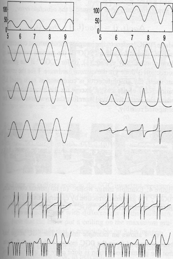
Figure 2: An analytical example function. (left) f(x) = 3x \sin(2\pi x) + 30 ; (right) f_\gamma(x) = p f(x)^\gamma , \gamma = 0.45 . (first row) original functions (second row) first derivatives; (third row) second derivatives; (fourth row) third derivatives; (fifth row) \Theta_{m12\gamma} ; (sixth row) \Theta_{m123\gamma} .
