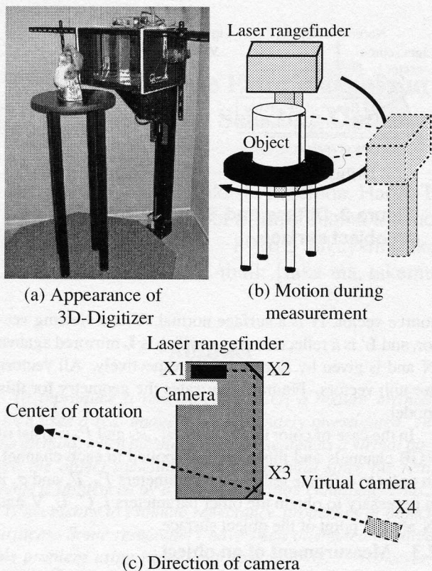
Figure 3. 3D-Digitizer.
