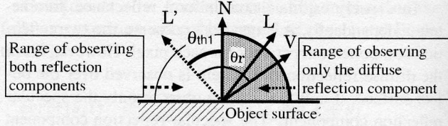
Figure 6. Observation of only the diffuse reflection component.
