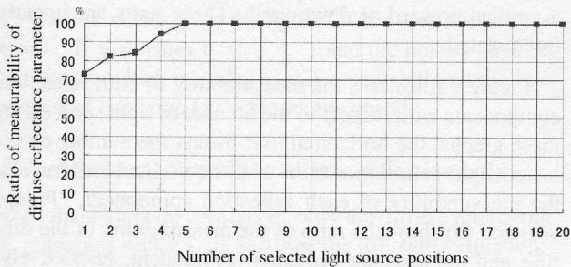
(a) Measurability of diffuse reflectance parameter
