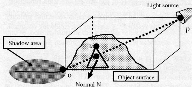
Figure 5. An illumination of detecting a self-shadow.
