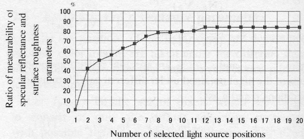
(b) Measurability of specular reflectance and surface roughness parameters
