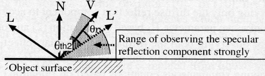
Figure 7. Observation of the specular reflection component strongly.
