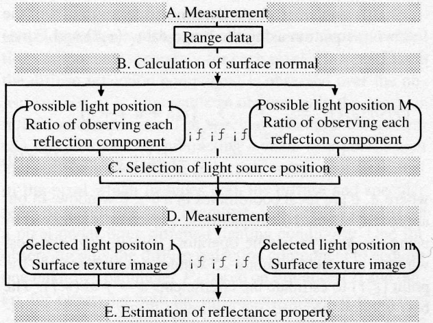
Figure 1. Flow diagram of estimating surface reflectance properties.
