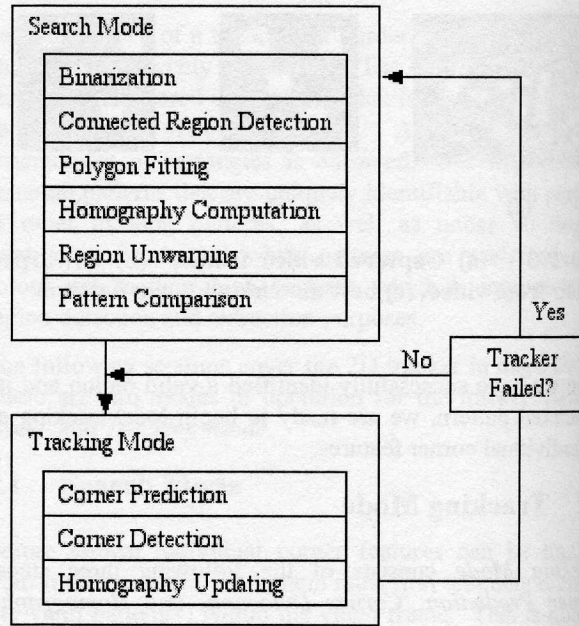
Figure 5 – Block diagram of the augmentation system
